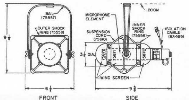
Figure 3 - Dimensions
