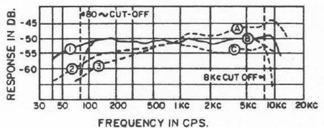
Figure 1 - Frequency Response
