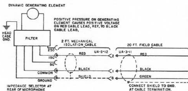
Figure 4 - Wiring Diagram
