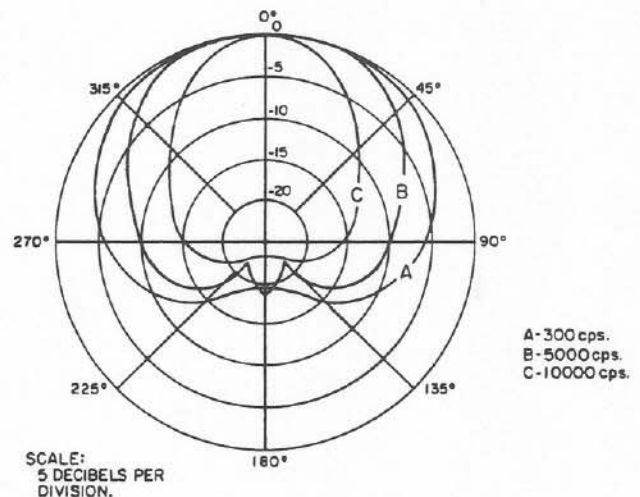
Figure 2 - Polar Pattern
